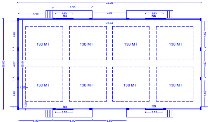
PLAN FOR 1040 MT WAREHOUSE SCALE 1:100
