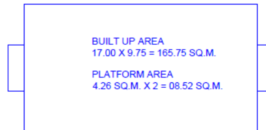
BUILT UP AREA SCALE: NTS
