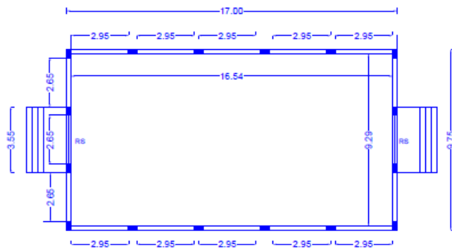
PLAN SCALE 1:100
